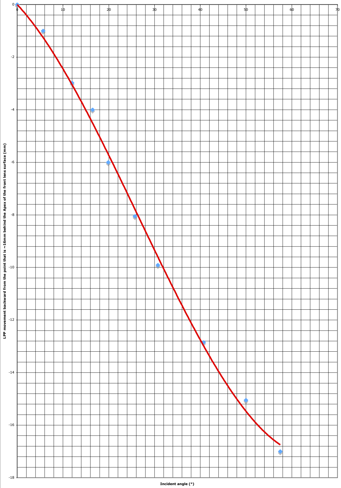
Movement of the LPP along the axis of the Samyang 14mm f2.8
