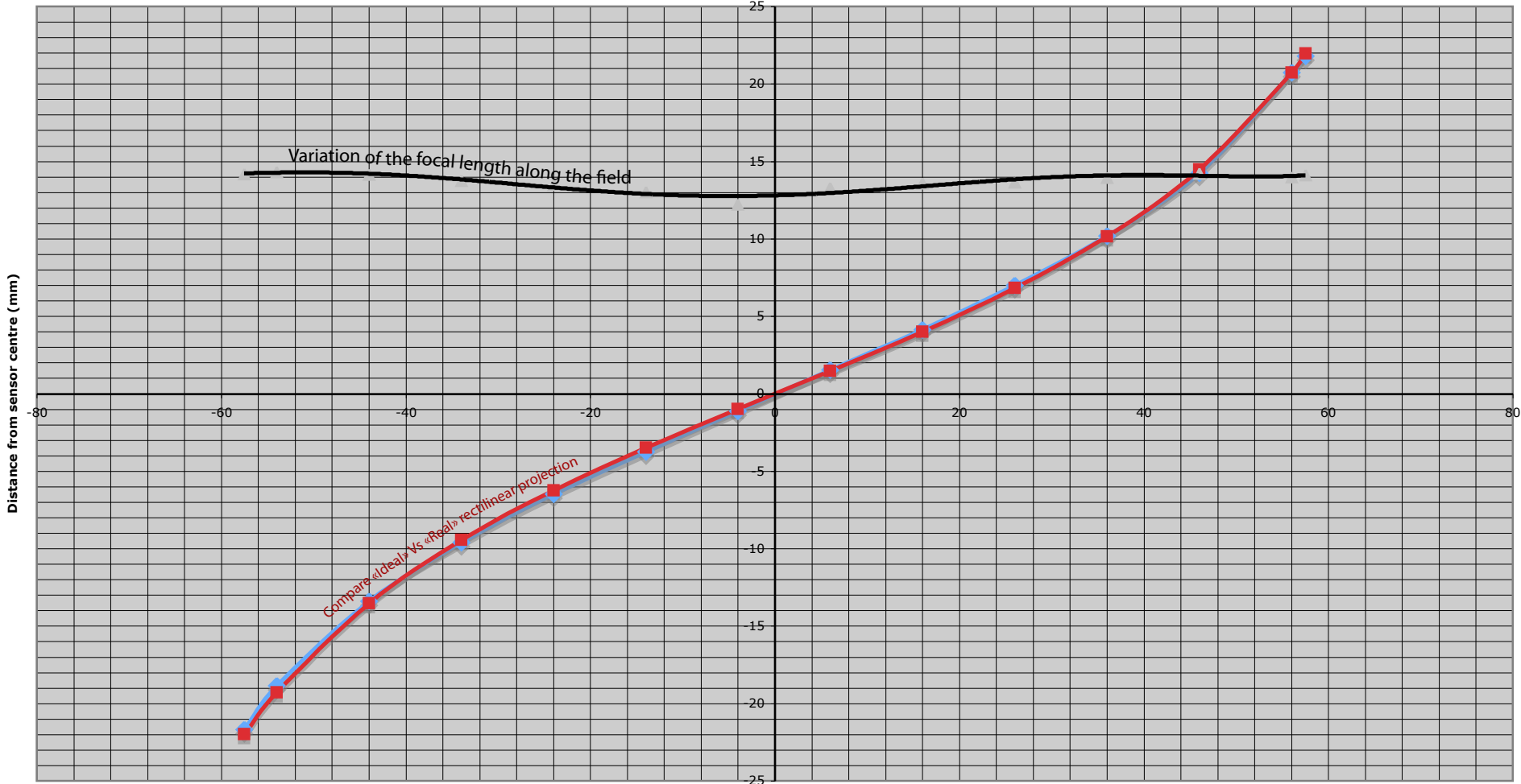
◆ 14mm Samyang ■ Ideal 14 mm rectilinear ▲ Focal length (mm) Vs Field Angle — Poly. (Focal length (mm) Vs Field Angle)
